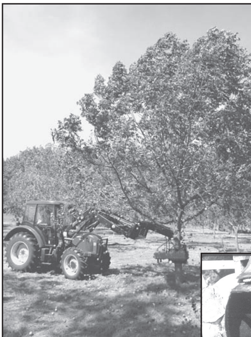
Fig. 13. (Left) A tree shaker mounted to a front-end loader is used to remove walnuts from the tree. Fig. 16. (Right) The tire and cage huller uses the force of a rotating tire to smash the hull against a rebar cage, removing hull from nut. Fig. 17. (Below) A homemade nut washer features rubberized stirring paddles. Fig. 18. (Below right) Nuts are spread on drying racks and allowed to air dry.
